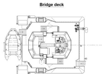
Bridge deck
