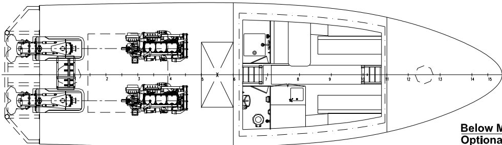
Below Maindeck Crew tender version
