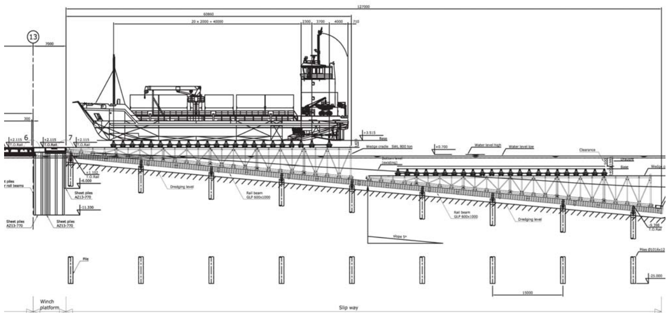
SLIPWAY SECTION
